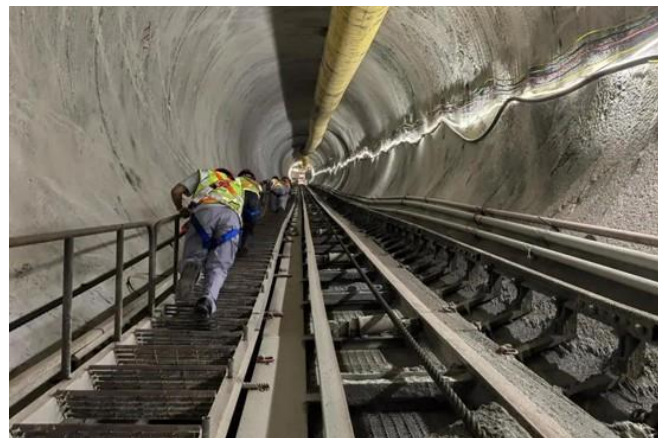
The 50 degree slope tunnelled by the TBM Tianyu
